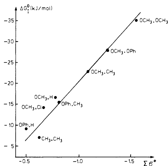
Figure 1. Correlation of the free energies of ionization ( \Delta G_1^\circ ) of para-substituted diarylmethyl chlorides 1-X, Y in \text{CD}_2\text{Cl}_2/\text{BCl}_3 at -70\text{ }^\circ\text{C} versus the sum of \sigma^+ values. The correlation equation ( r = 0.980 ) is \Delta G_1^\circ = 5 + 26\Sigma\sigma^+ (kJ/mol).
